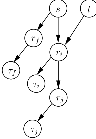
Figure 5.15. This shows the different types of feedback elements. Reference r_f is a task-independent reference, typically for force-based controllers. Reference r_i is a task dependent reference, and r_j is a reference dependent on r_i .
