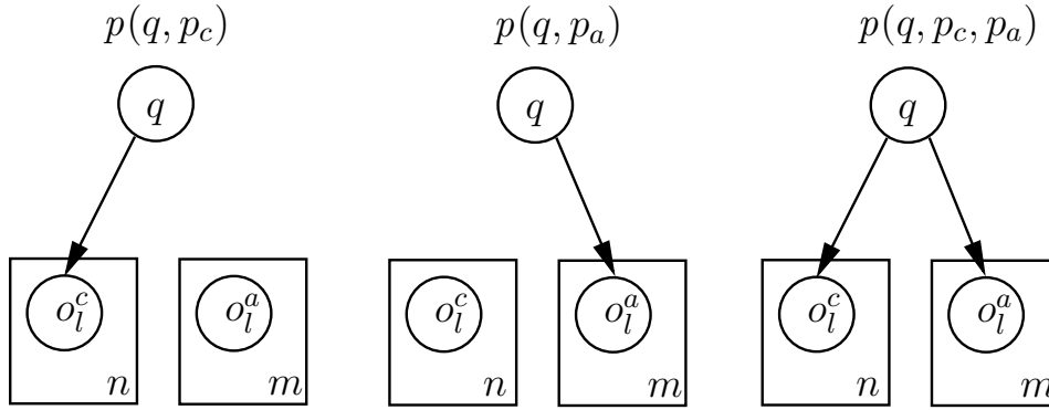
Figure 5.17. This shows the different possible relationships between q and the feature types. The lack of an arrow between nodes indicates no statistical relationship exists between the variables.
