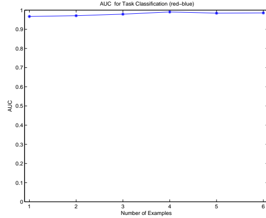
Figure 5.9. This shows the AUC (area under the curve) for the ROC curves presented in Figure 5.8.
