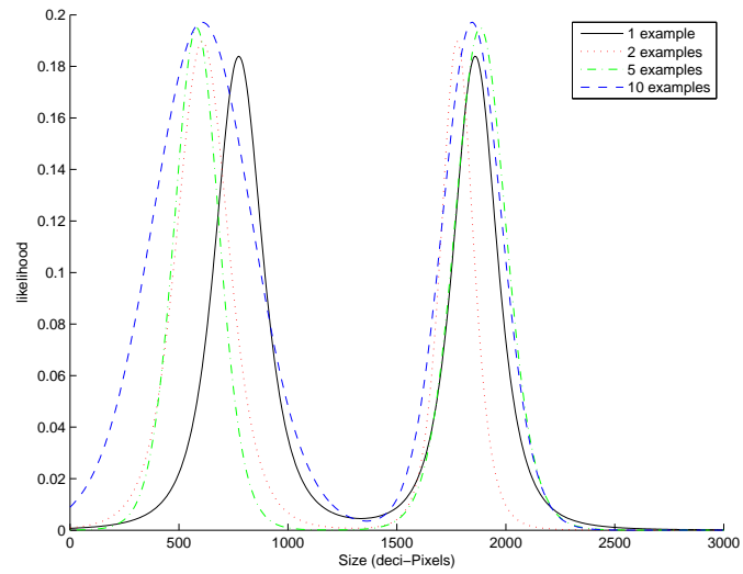
Figure 5.5. The posterior distribution over size after different numbers of training examples. The distribution is bimodal, with the peak on the left accounting for Small objects, and the peak on the right describes Large objects.
