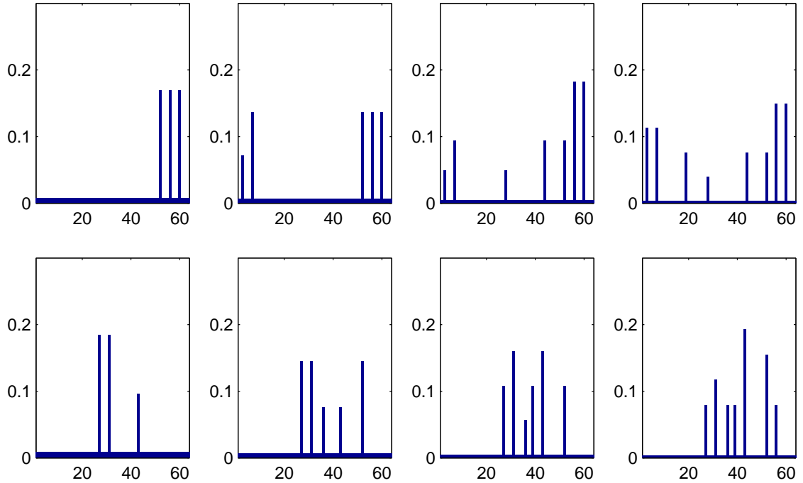
Figure 5.12. This shows the evolution of the probability mass functions; the x-axis corresponds to the set of 64 discrete colors. The top row shows the Red/Black category, and the bottom shows Blue/White. Each column, from left to right, show the effect of an additional example provided by the demonstrator.
