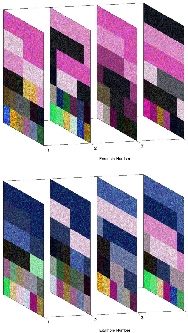
Figure 5.13. Colors generated from each pmf, as new examples are provided. Each slice represents a collection of 36 samples from the posterior distribution. Each sample represents one of 64 different HSV regions, and the color of the region is shown by pixels taken uniformly from the region. The slices from left to right show the effect of an additional training example. The top row corresponds to the Red/Black task, and the bottom to Blue/White. As examples are added, each slice shows the posterior distribution becomes closer to the true Red/Black or Blue/White distribution.
