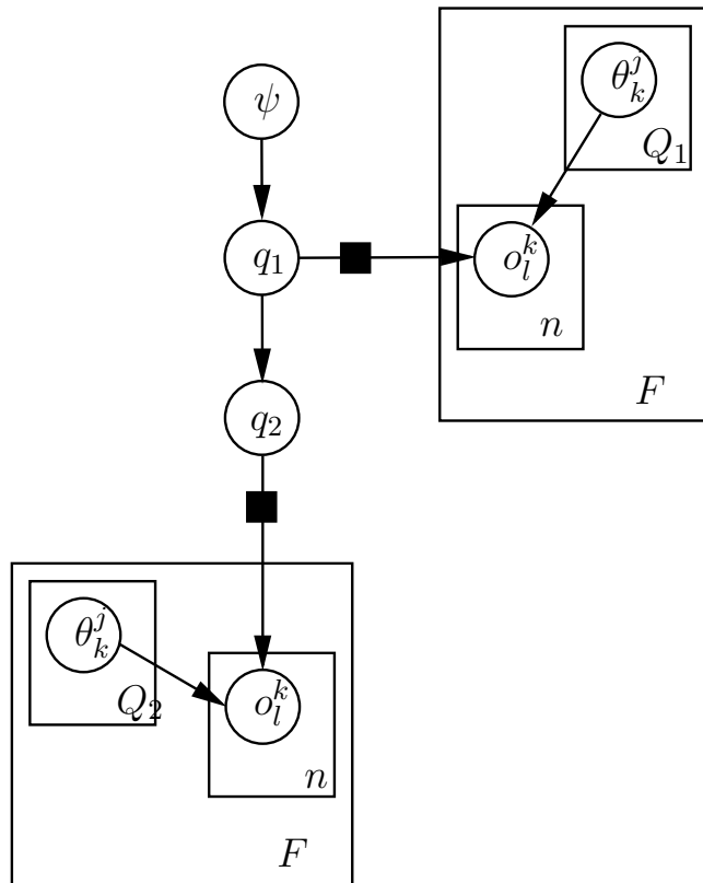
Figure 5.16. A generic feature model for a schema with two references.
