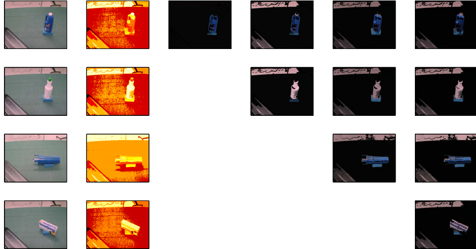
Figure 5.14. This figure shows how the model changes incrementally. The left column shows an image of the object presented for training. The second column shows the object after color quantization. The remaining images are constructed from the quantized image by filling in pixels based on the likelihood of the segments color according to the learned distribution.
