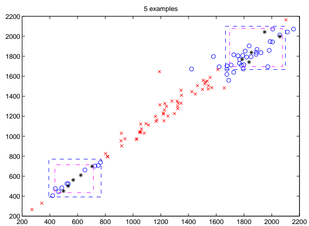
Figure 5.11. The posterior classification of task relevance.
